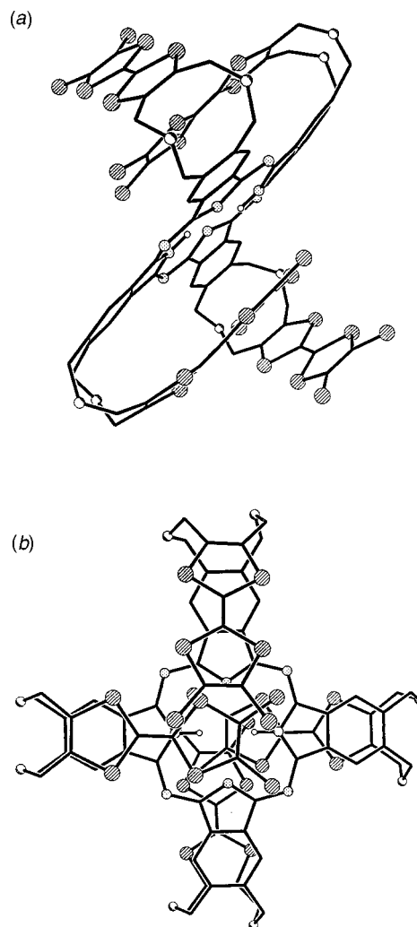
Fig. 6 Energy-minimised structure of compound 14 (side chains omitted for clarity): (a) view showing folding of the molecule around the Pc ring; (b) view onto the plane of the Pc ring
